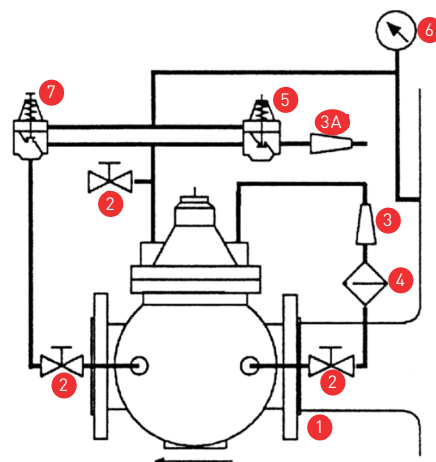
G-FPV-88 Hydraulic Surge Anticipating Control Valve
