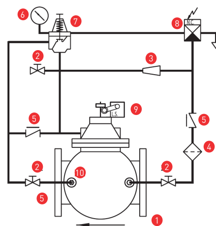
G-FPV-60 Pressure Reducing Control Valve
