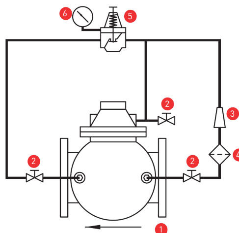
G-FPV-60 Pressure Reducing Control Valve
